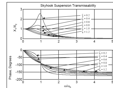
Figure 2.4. Ideal Skyhook Transmissibility.
