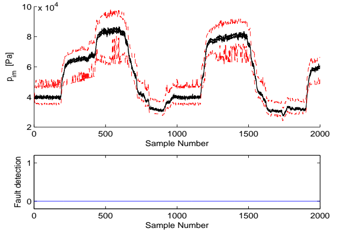
Fig. 5. Second scenario without faults. The upper plot shows measured and estimated manifold pressure.
