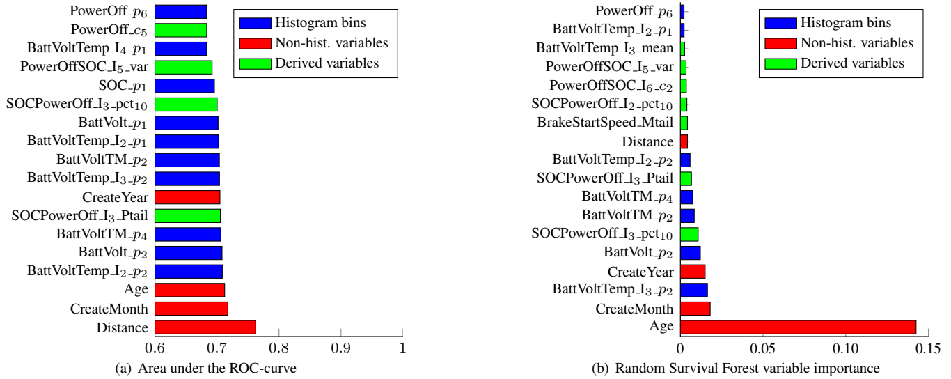
Figure 14. Individual predictive power for the most influential variables based on the area under the ROC-curve and ranking based on variable importance in the random survival forest.
