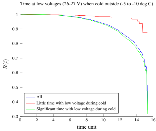
Figure 4. Reliability function estimate for vehicles with different amount of time with low battery voltage during cold ambient temperatures.
